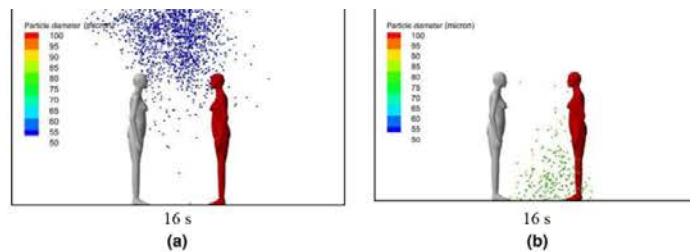
FIGURE 7 Computer simulated dispersion of large expiratory droplets (initial size, 100 \mu\text{m} in diameter) due to normal breathing in a mixing ventilated room with a low (35% \text{O}_2 and a high (95%) RH (a) Case 8 [100, mixing, 5.6 ACH, 35%, 0.8 m, 0] (b) Case 9 [100, mixing, 5.6 ACH, 95%, 0.8 m, 0] at 6 instances (6, 10, 14, and 16 s)
